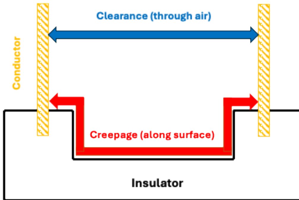
Figure 2: Creepage and clearance distance.
